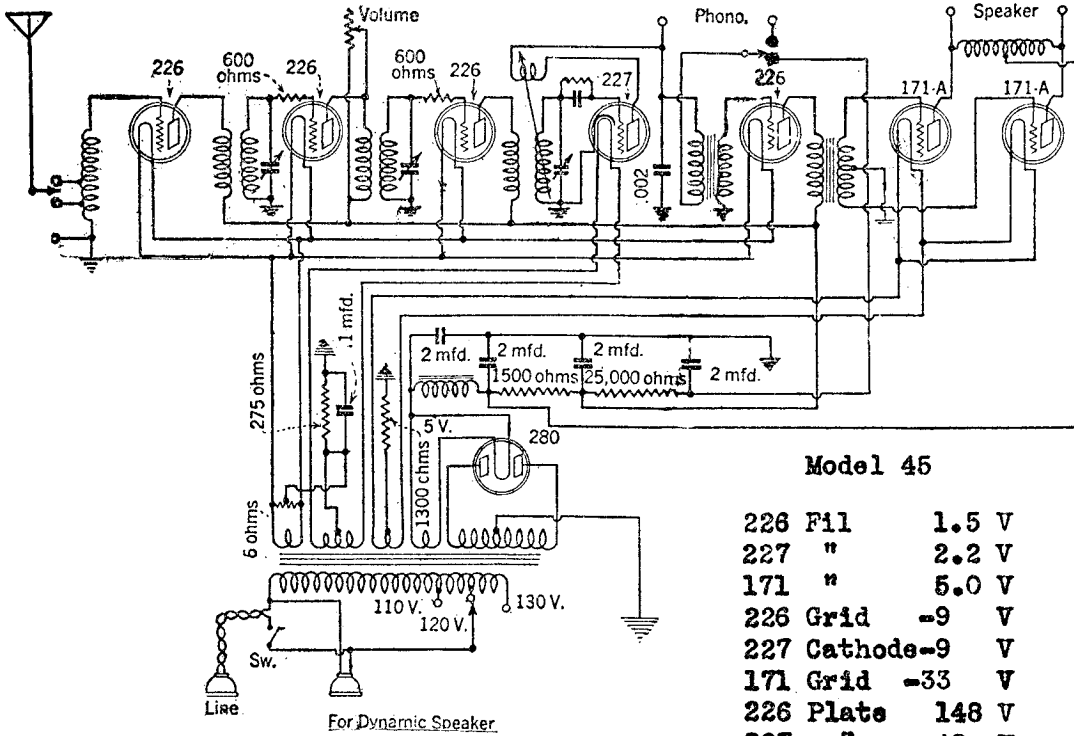
Model Arborphone 45
